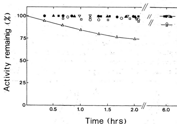
Fig. 1. Photodynamic inactivation of enzymes in presence of 2 \times 10^{-4} M 8-MOP under oxygen. Bovine ( \square — \square ) or tuna ( \blacktriangle — \blacktriangle ) liver glutamate dehydrogenase, 2.8 \times 10^{-6} M in phosphate buffer 0.05 M, 0.9% NaCl, pH 7.4. Rabbit muscle enolase ( \blacksquare — \blacksquare ), 1.2 \times 10^{-6} M in Tris-HCl buffer 0.05 M, 0.9% NaCl, 10^{-3} M 2-mercaptoethanol, pH 7.5. Yeast 6-phosphogluconate dehydrogenase ( \circ — \circ ), 1 \times 10^{-6} M, in Tris-HCl buffer 0.1 M, 5 \times 10^{-5} M EDTA, 10^{-3} M 2-mercaptoethanol, pH 7.4. Thermolysin, ( \bullet — \bullet ), 2.2 \times 10^{-5} M, in Tris-HCl buffer 0.1 M, 10^{-2} M \text{CaCl}_2 , pH 7.2. Hen egg white lysozyme ( \triangle — \triangle ), 5 \times 10^{-5} M, in phosphate buffer 0.01 M, 0.9% NaCl, pH 7.2. Ribonuclease A ( \nabla — \nabla ) 8 \times 10^{-5} M, in ammonium acetate buffer 0.05 M, pH 5.
